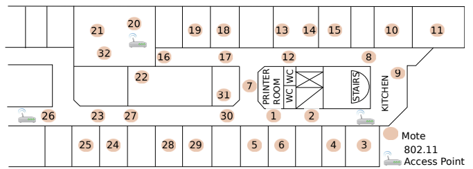
Fig. 1. Our testbed deployment consisting of 32 nodes. Three WiFi access points per floor, microwave ovens, and people moving in and in-between offices create different types of interference.
